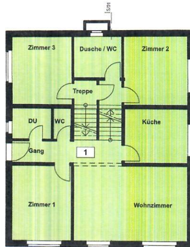
1 4 1/2 Zi-WHG Nr.1 Nettofläche103.75m 2
